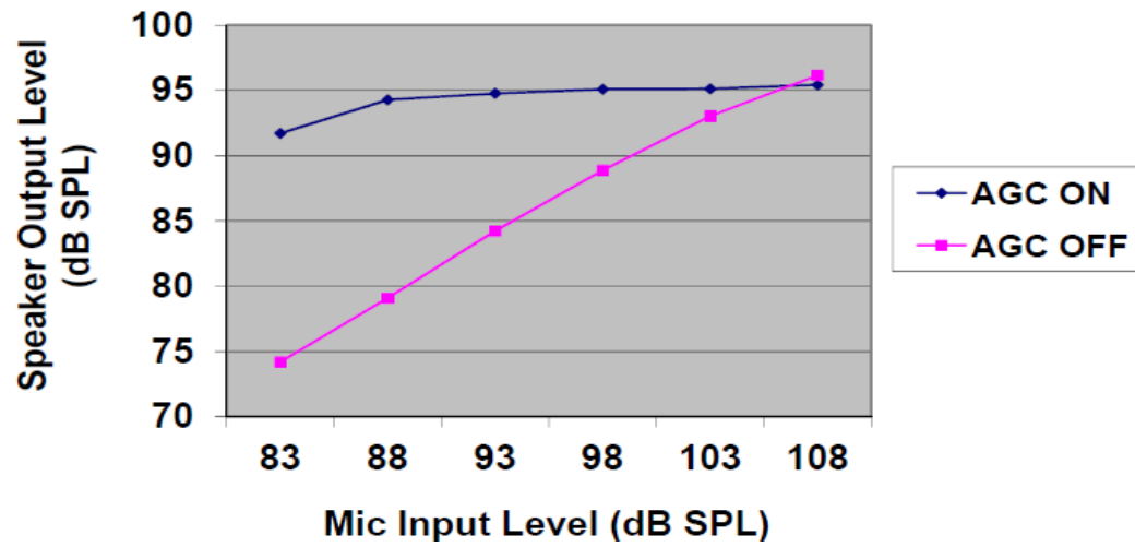
Figure 1 AGC Response
